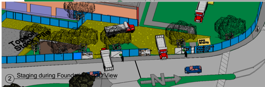
① Staging during Foundations - Plan View
